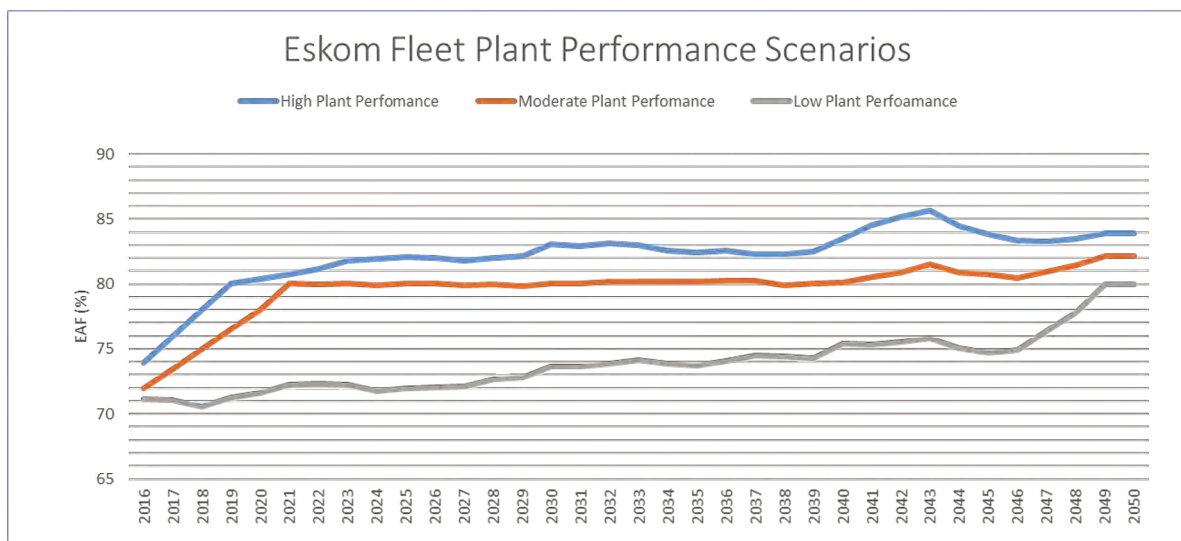
Figure 3: Eskom existing fleet plant performance
