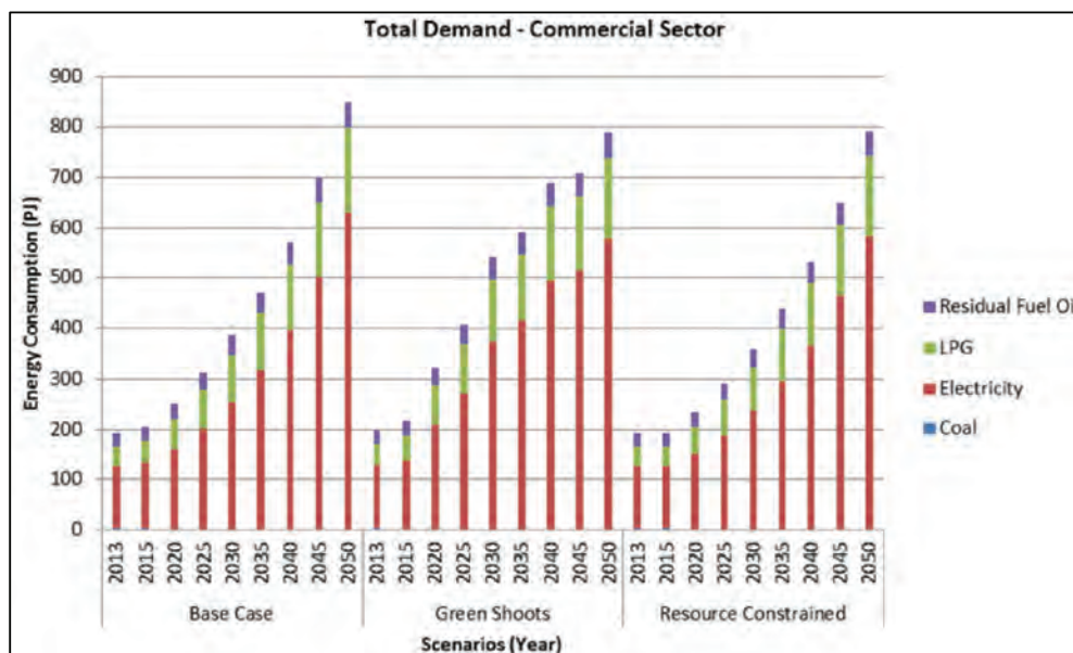
Figure 0-7: Projected demand in the commercial sector
